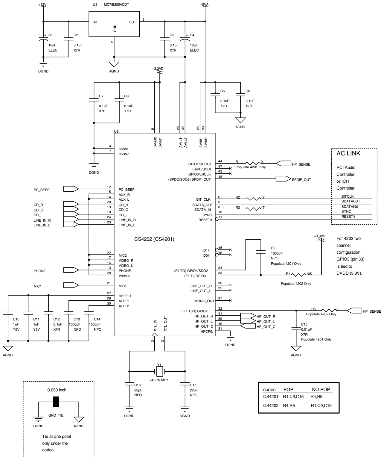
Figure 3. CS4202
