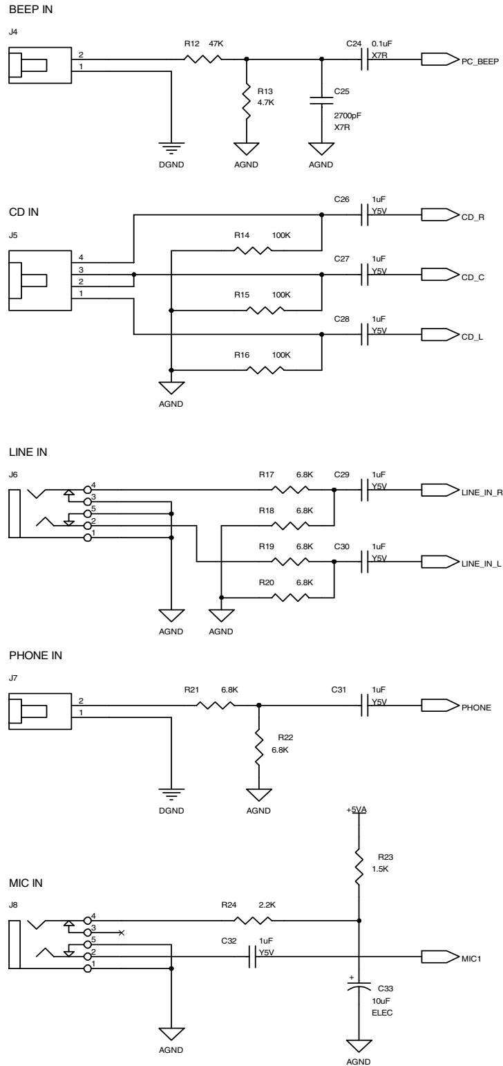
Figure 2. Audio Inputs
